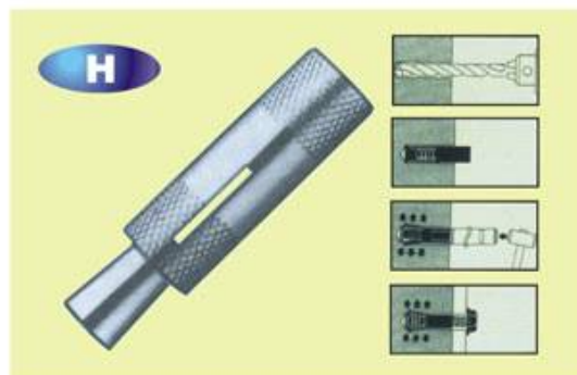
內牙膨脹螺絲 GRIP ANCHOR
